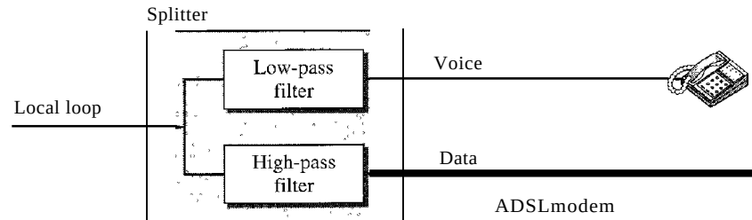
Figure 9.12 ADSL modem
