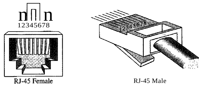
Figure 7.5 UTP connector
