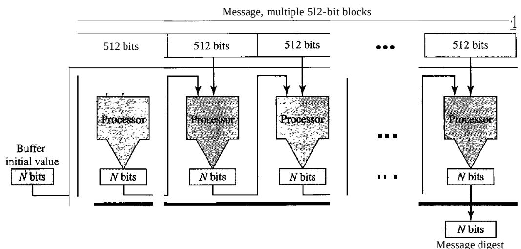
Figure 31.7 Message digest creation
