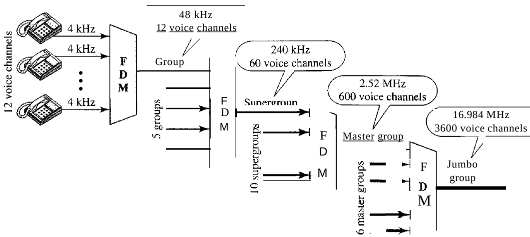
Figure 6.9 Analog hierarchy
