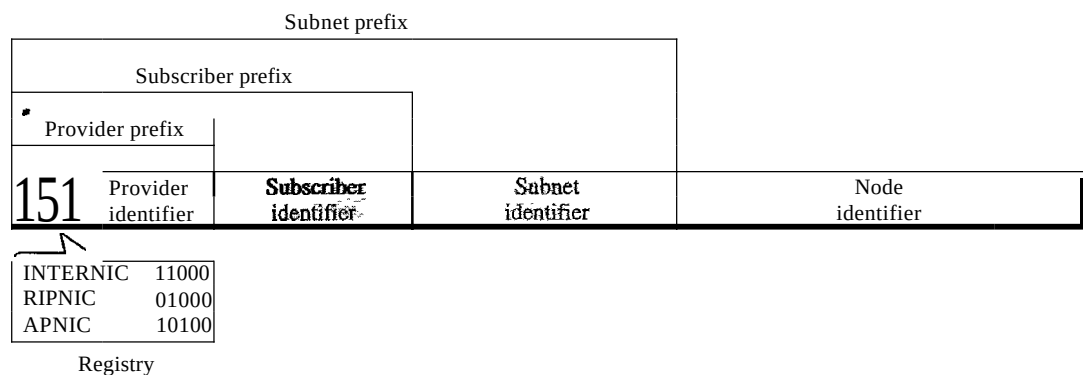
Figure 19.16 Prefixes for provider-based unicast address
